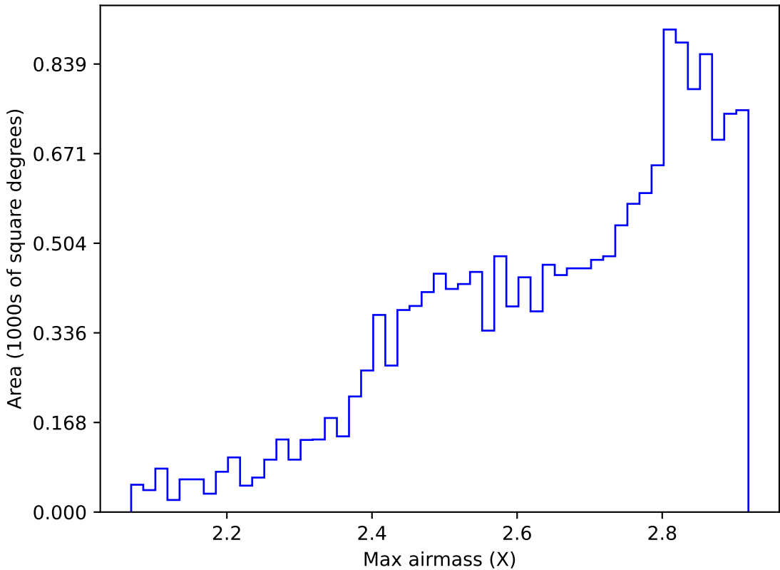
roll_pause_mjdp120_v3.4_10yrs WFD all bands: Max airmass
