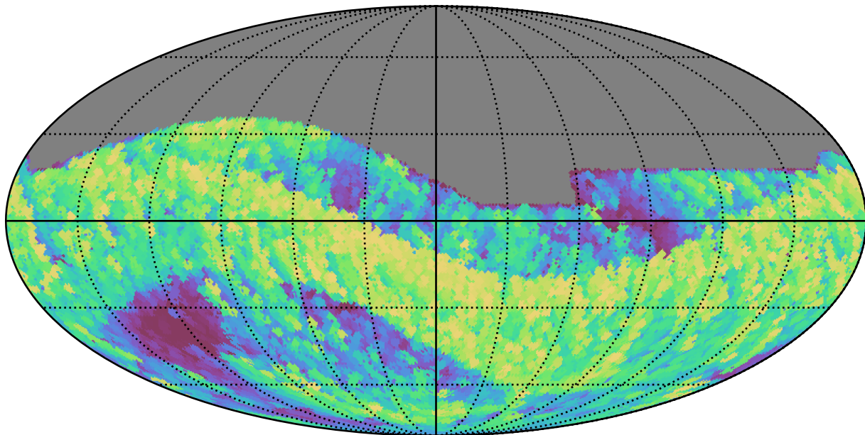
roll_pause_mjdp120_v3.4_10yrs All sky z band: Max airmass
