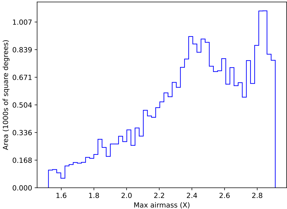
roll_pause_mjdp120_v3.4_10yrs All sky z band: Max airmass
