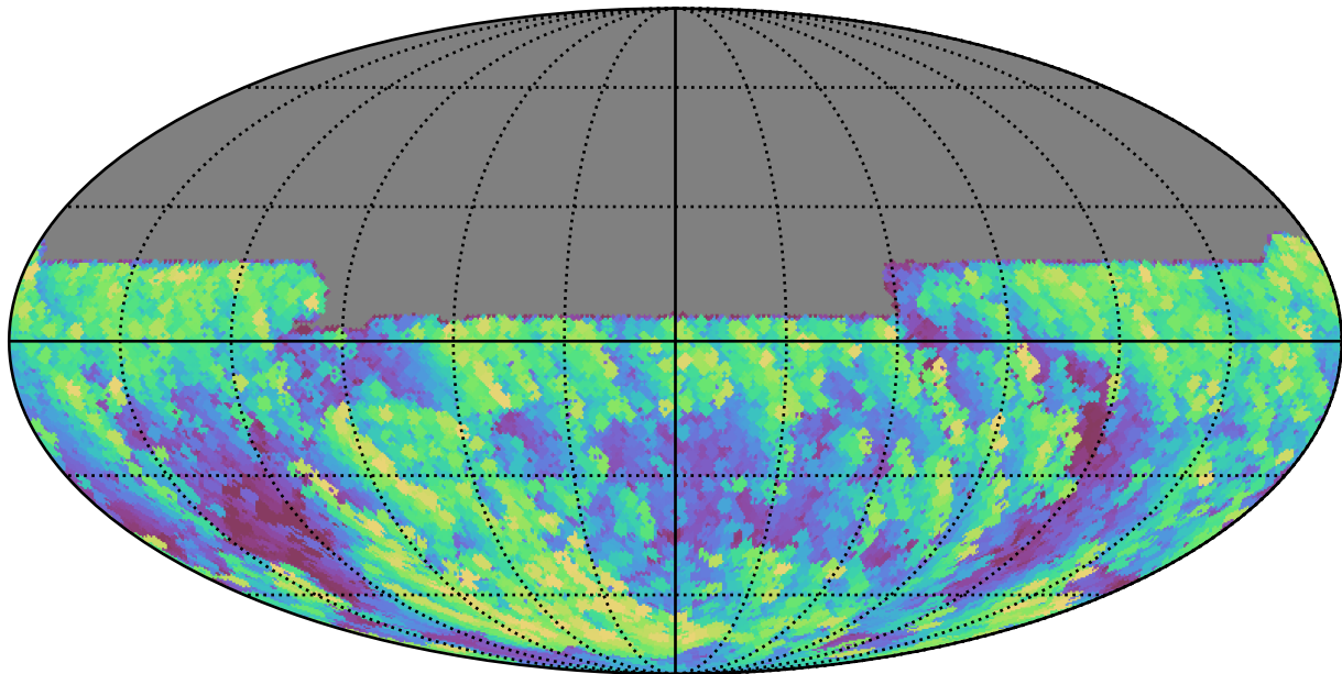
roll_pause_mjdp120_v3.4_10yrs All sky y band: Max airmass
