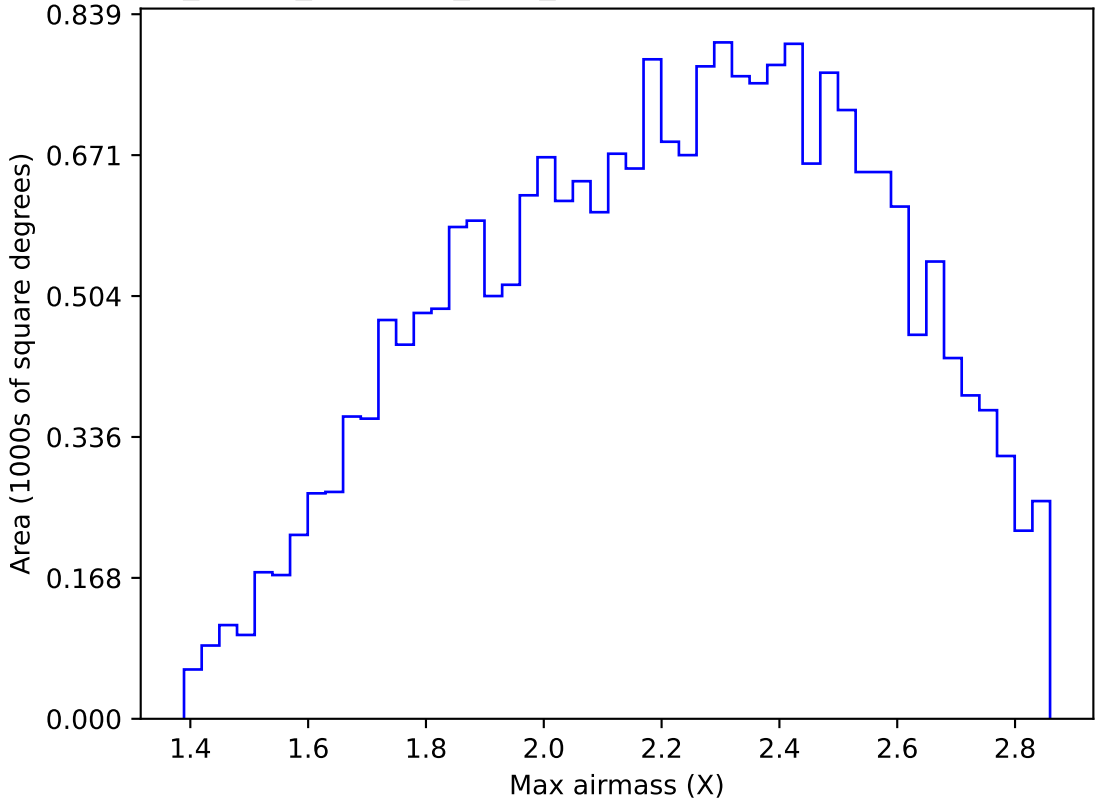
roll_pause_mjdp120_v3.4_10yrs All sky y band: Max airmass
