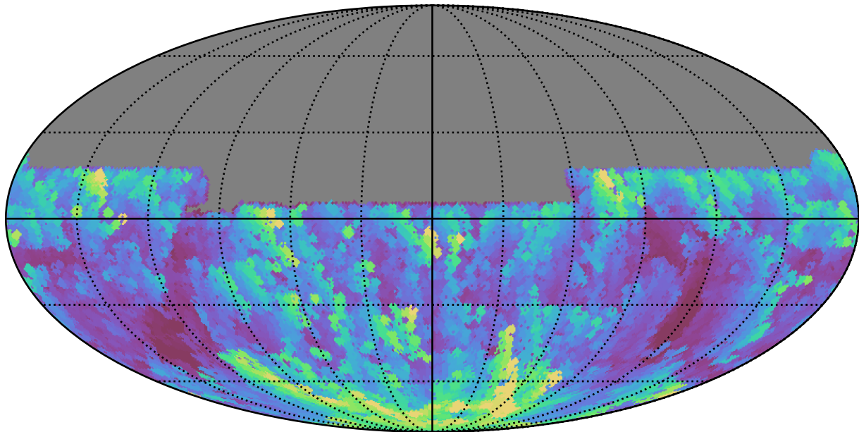
roll_pause_mjdp120_v3.4_10yrs All sky u band: Max airmass
