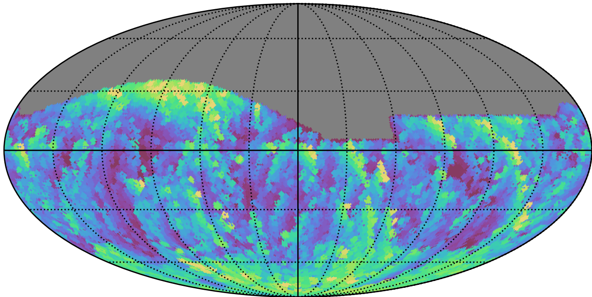
roll_pause_mjdp120_v3.4_10yrs All sky g band: Max airmass
