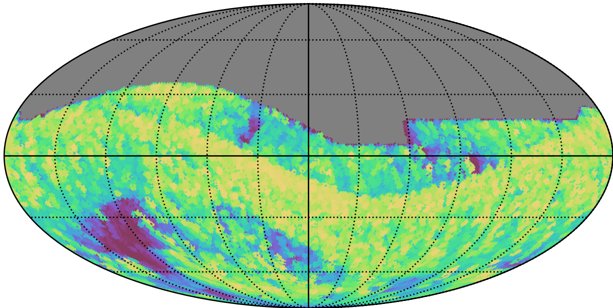
roll_pause_mjdp120_v3.4_10yrs All sky all bands: Max airmass
