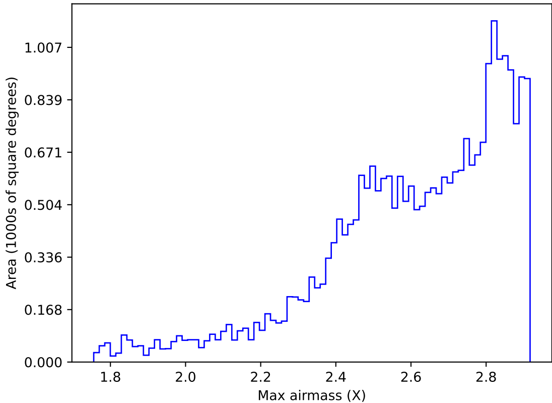
roll_pause_mjdp120_v3.4_10yrs All sky all bands: Max airmass
