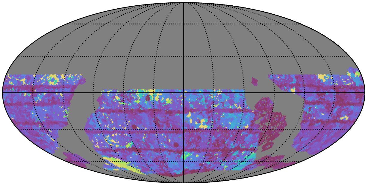
roll_pause_mjdp120_v3.4_10yrs WFD z band: Max Inter-Night Gap
