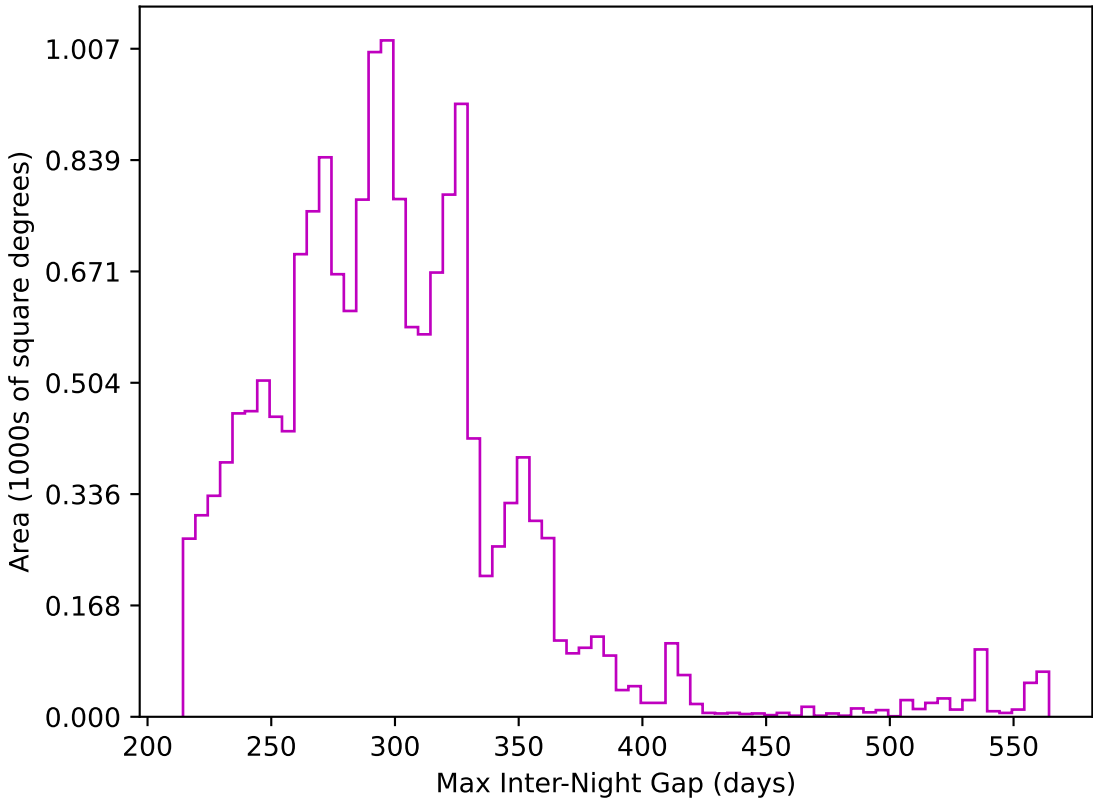
roll_pause_mjdp120_v3.4_10yrs WFD z band: Max Inter-Night Gap
