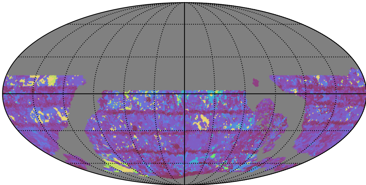
roll_pause_mjdp120_v3.4_10yrs WFD y band: Max Inter-Night Gap
