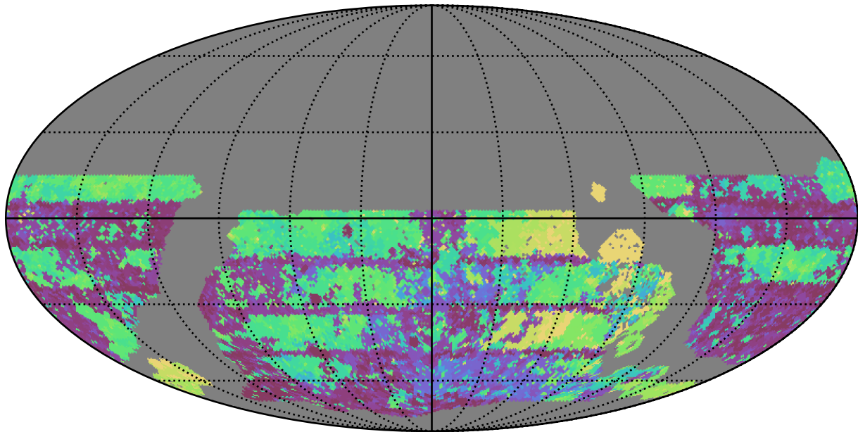
roll_pause_mjdp120_v3.4_10yrs WFD u band: Max Inter-Night Gap
