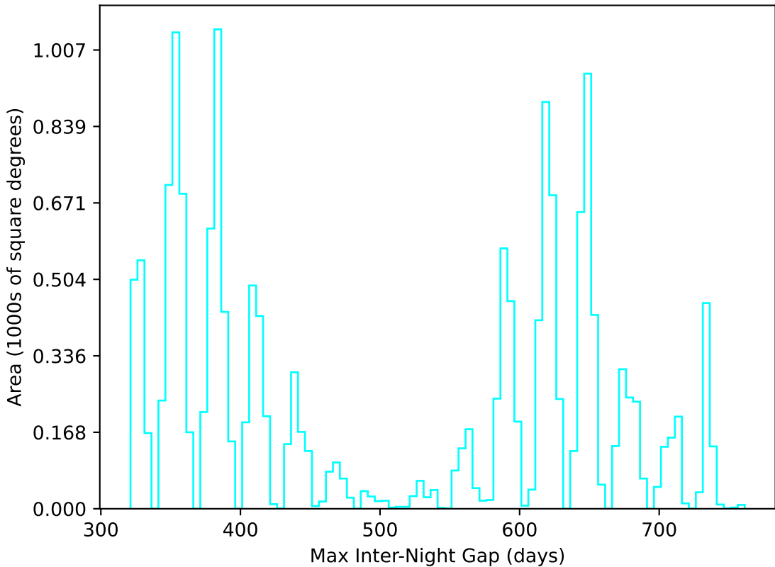
roll_pause_mjdp120_v3.4_10yrs WFD u band: Max Inter-Night Gap
