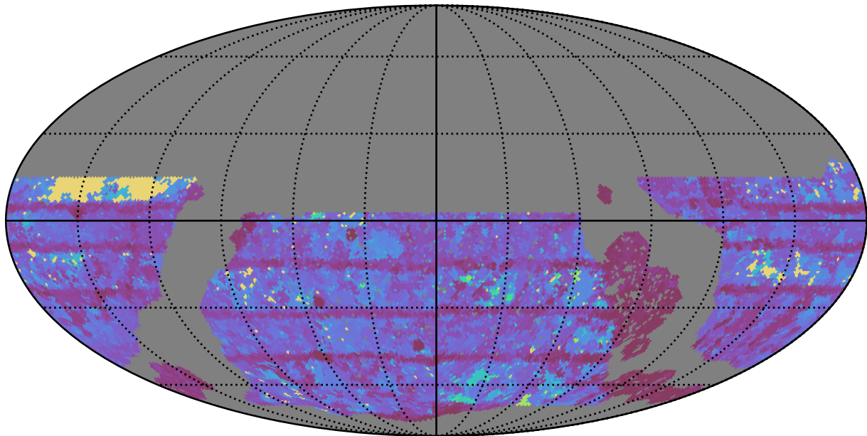
roll_pause_mjdp120_v3.4_10yrs WFD r band: Max Inter-Night Gap
