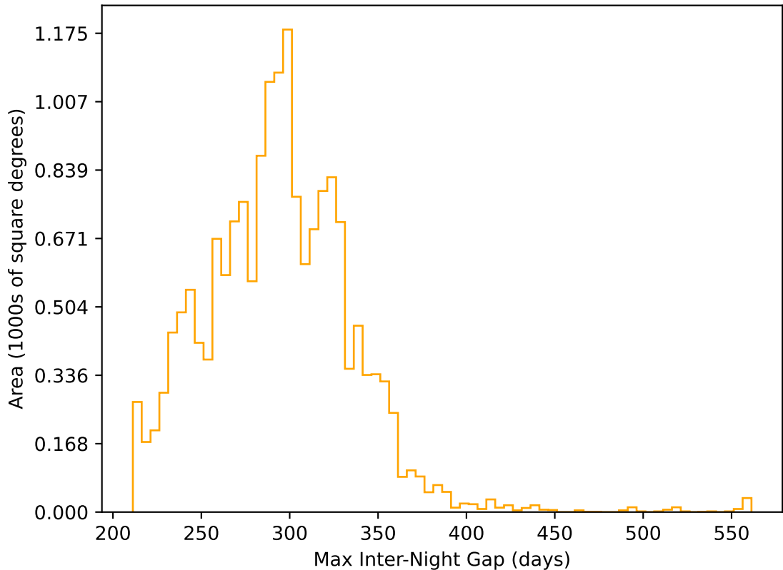
roll_pause_mjdp120_v3.4_10yrs WFD r band: Max Inter-Night Gap
