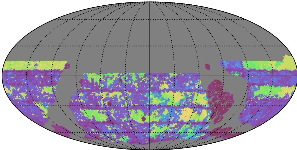
roll_pause_mjdp120_v3.4_10yrs WFD g band: Max Inter-Night Gap
