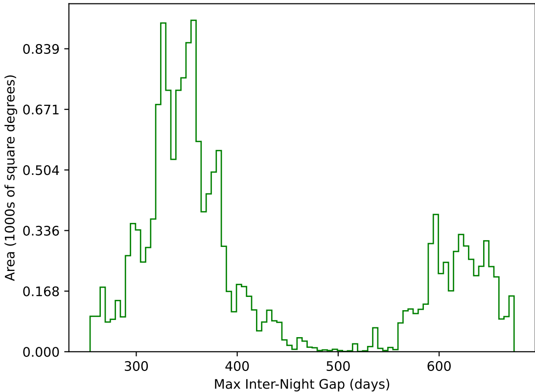
roll_pause_mjdp120_v3.4_10yrs WFD g band: Max Inter-Night Gap
