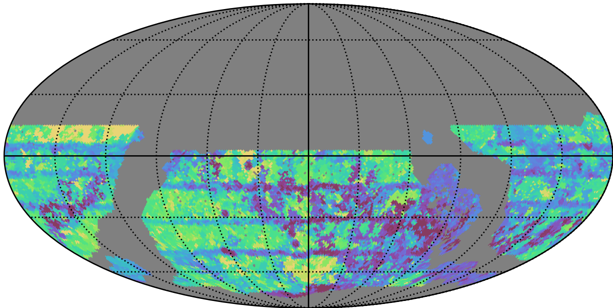
roll_pause_mjdp120_v3.4_10yrs WFD all bands: Max Inter-Night Gap
