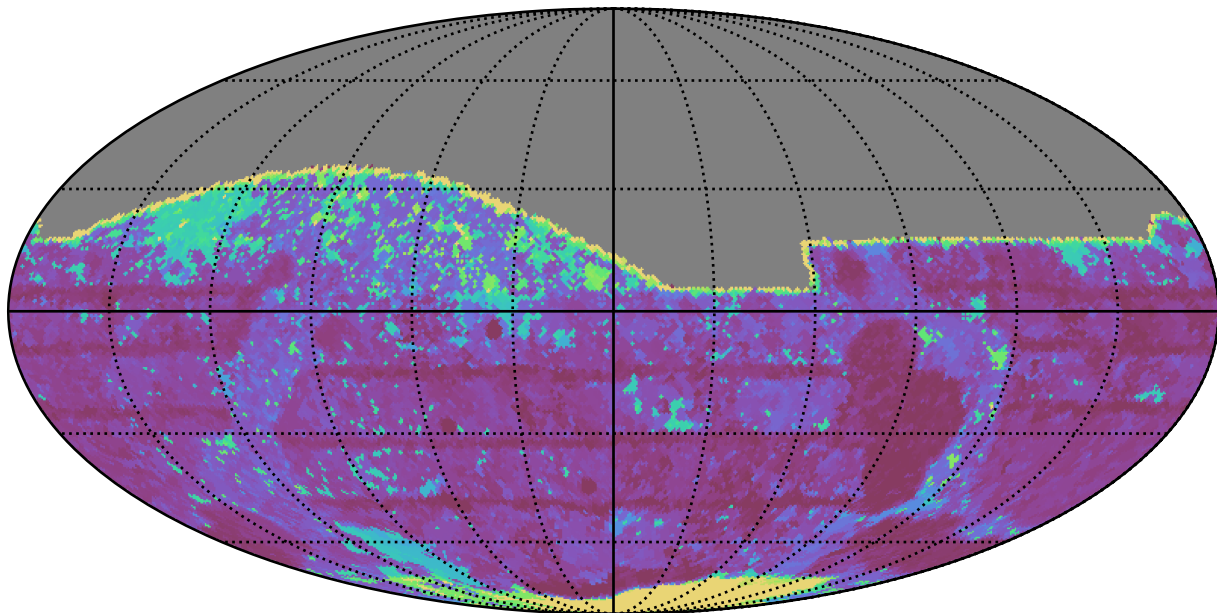
roll_pause_mjdp120_v3.4_10yrs All sky z band: Max Inter-Night Gap
