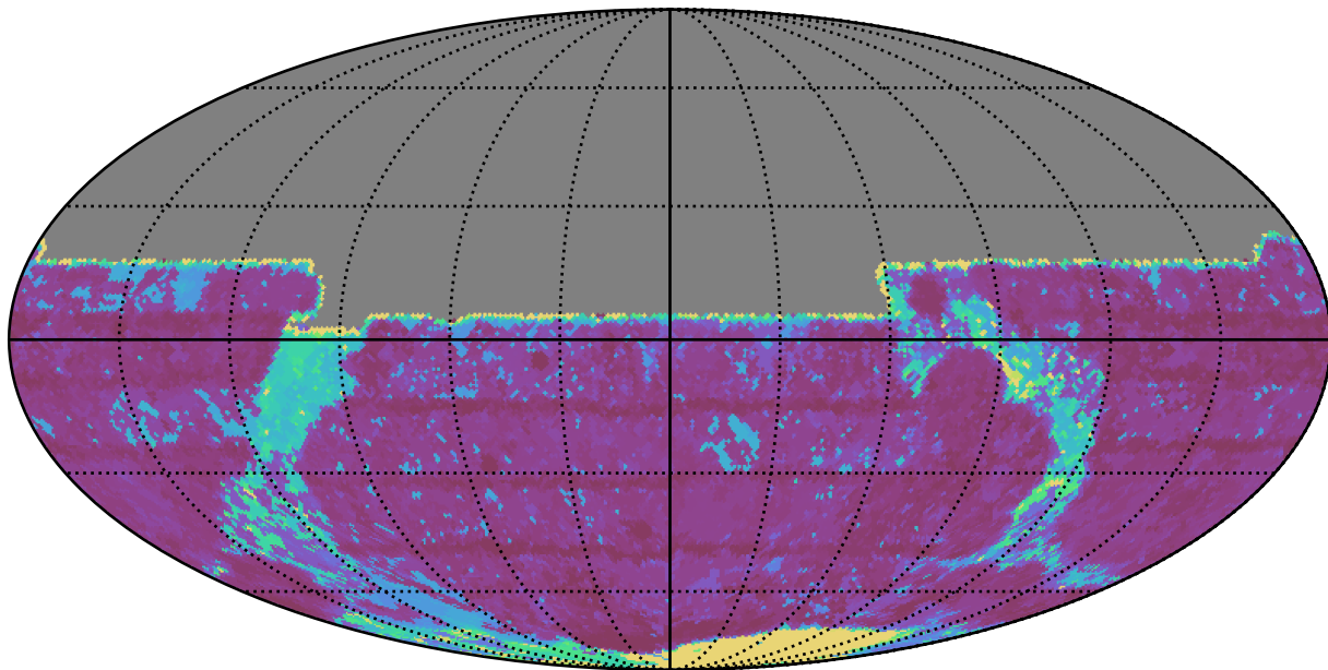
roll_pause_mjdp120_v3.4_10yrs All sky y band: Max Inter-Night Gap
