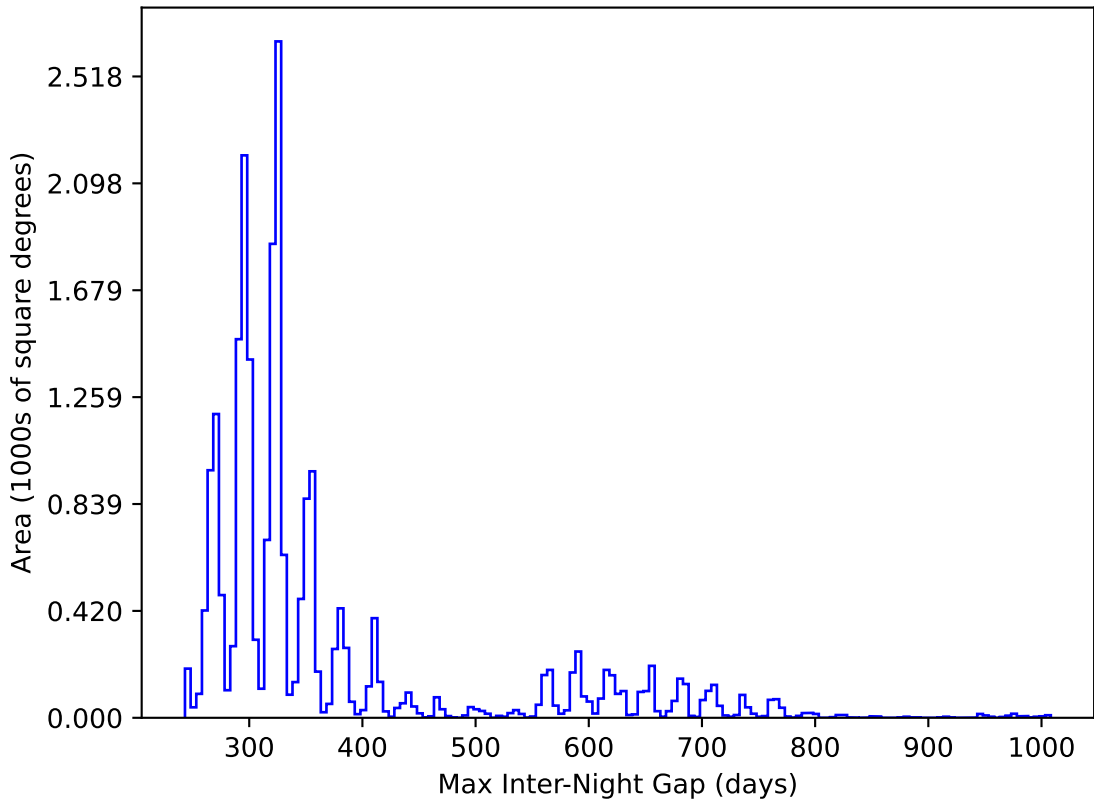
roll_pause_mjdp120_v3.4_10yrs All sky y band: Max Inter-Night Gap
