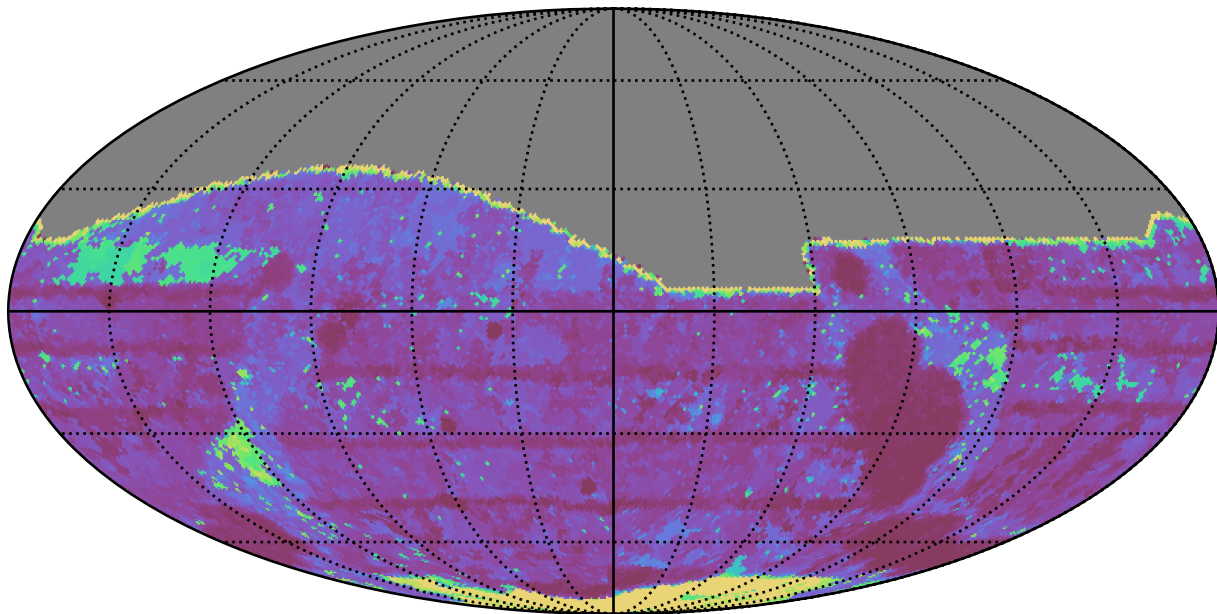
roll_pause_mjdp120_v3.4_10yrs All sky r band: Max Inter-Night Gap
