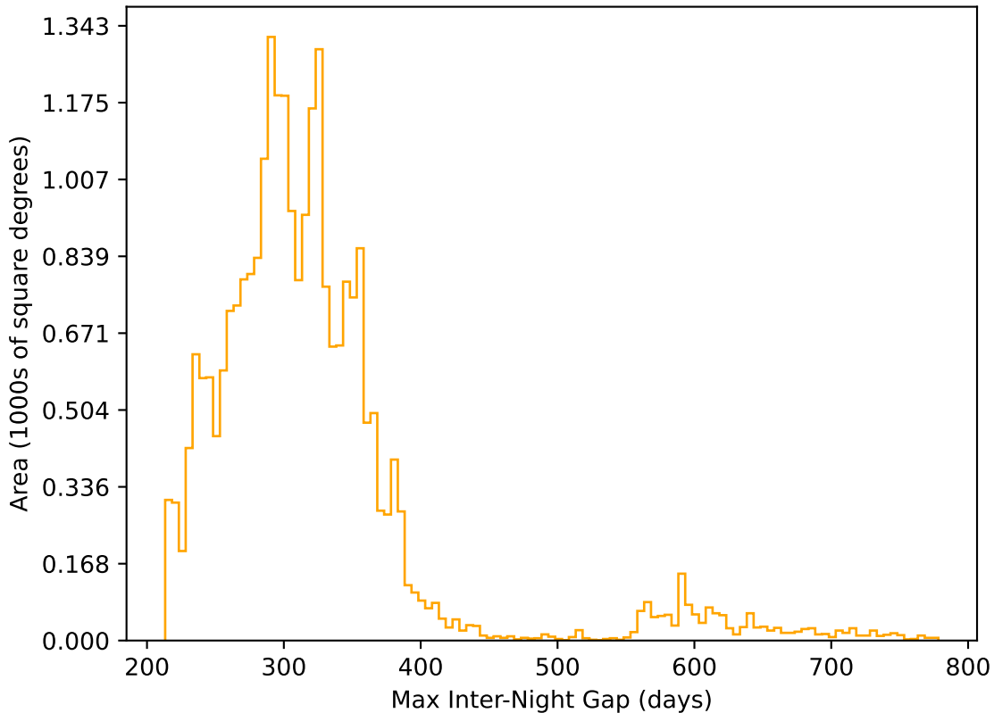
roll_pause_mjdp120_v3.4_10yrs All sky r band: Max Inter-Night Gap
