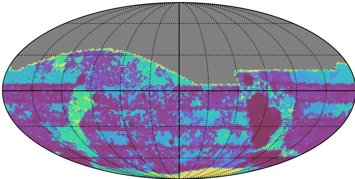
roll_pause_mjdp120_v3.4_10yrs All sky g band: Max Inter-Night Gap
