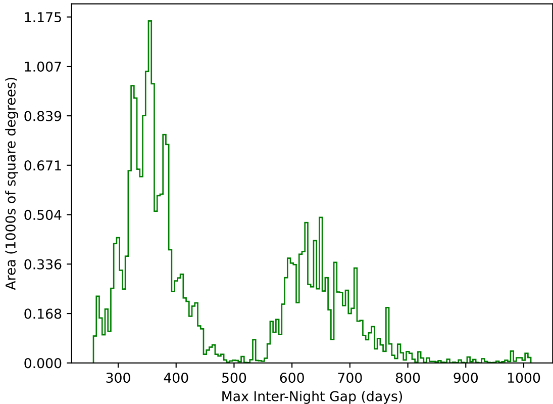
roll_pause_mjdp120_v3.4_10yrs All sky g band: Max Inter-Night Gap
