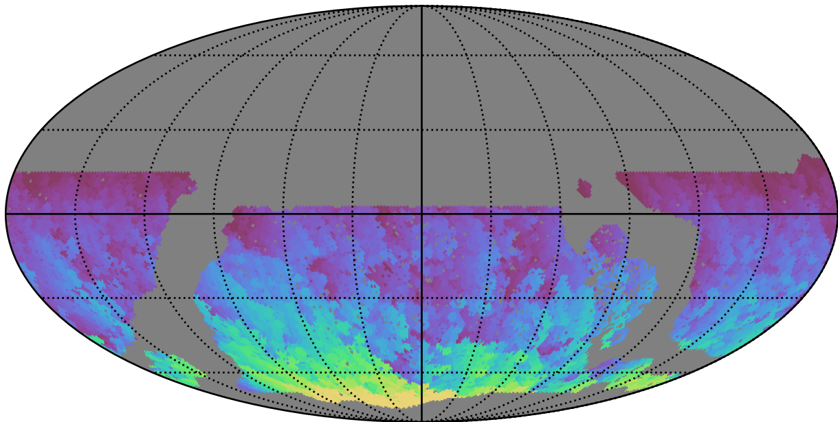
roll_pause_mjdp120_v3.4_10yrs WFD y band: Max HA
