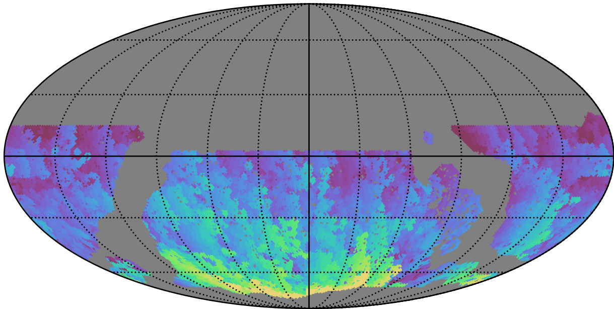
roll_pause_mjdp120_v3.4_10yrs WFD u band: Max HA
