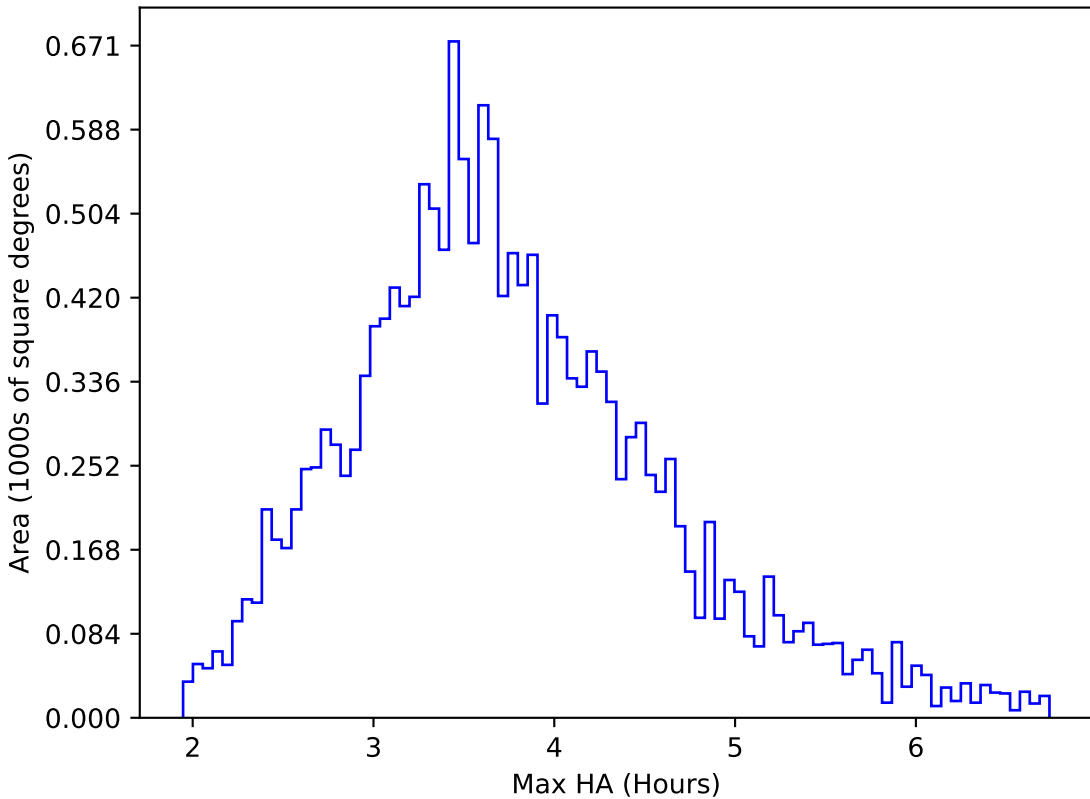
roll_pause_mjdp120_v3.4_10yrs WFD u band: Max HA
