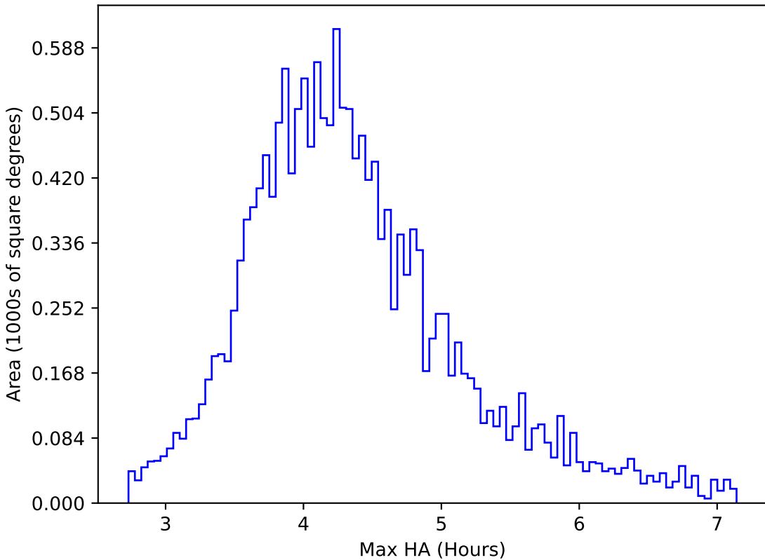
roll_pause_mjdp120_v3.4_10yrs WFD r band: Max HA
