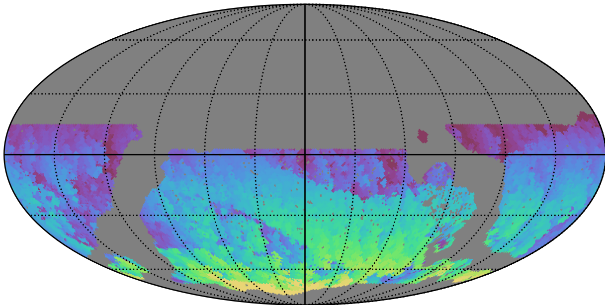
roll_pause_mjdp120_v3.4_10yrs WFD i band: Max HA
