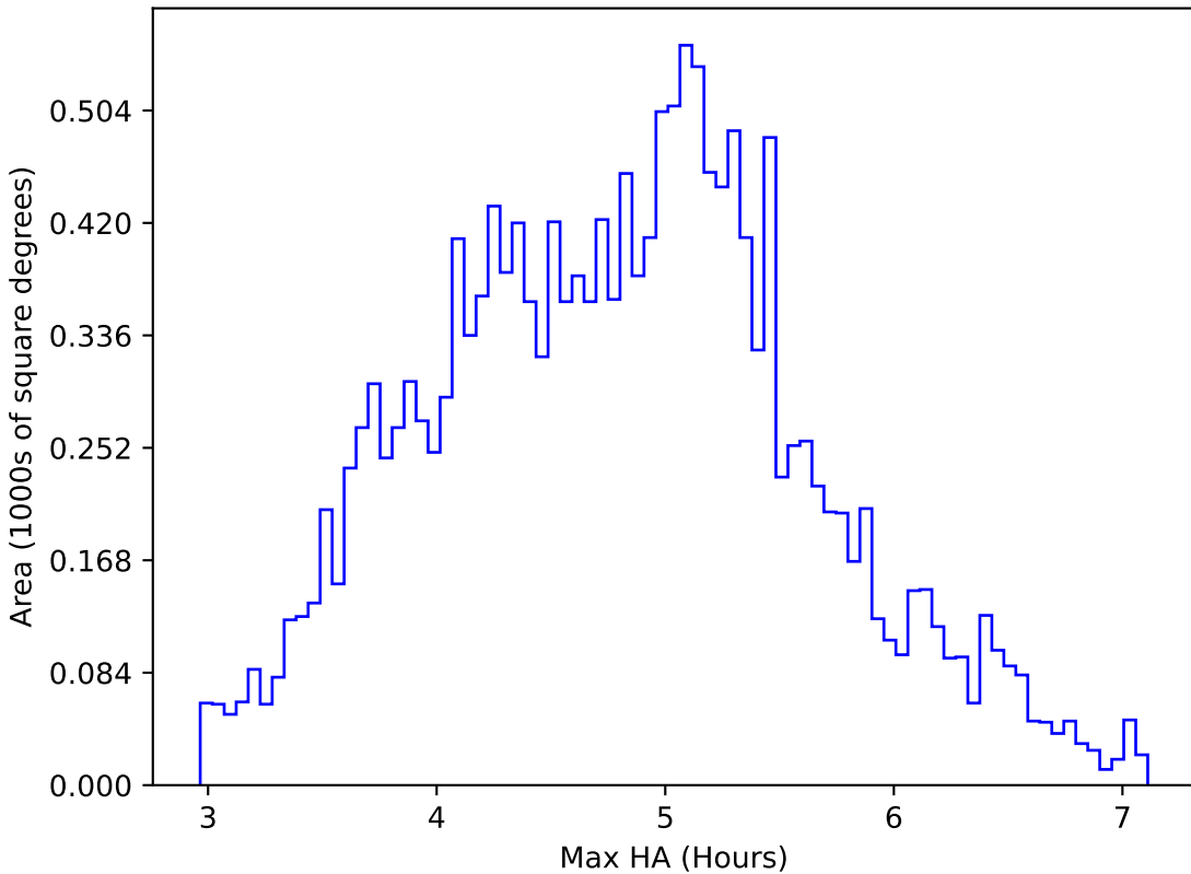
roll_pause_mjdp120_v3.4_10yrs WFD i band: Max HA
