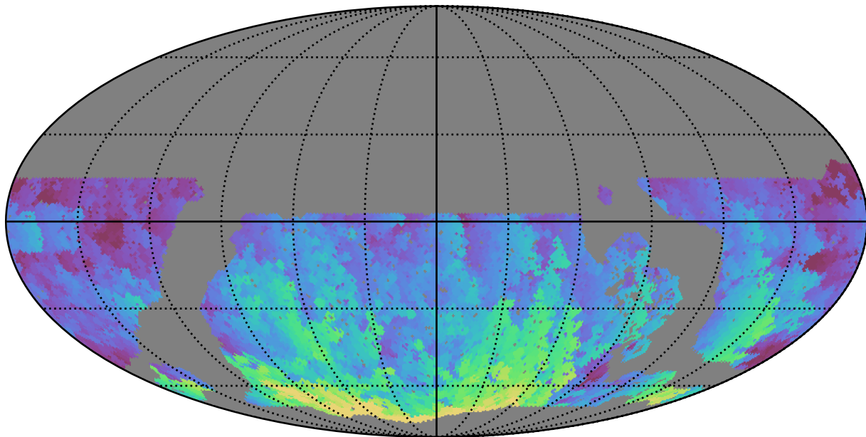
roll_pause_mjdp120_v3.4_10yrs WFD g band: Max HA
