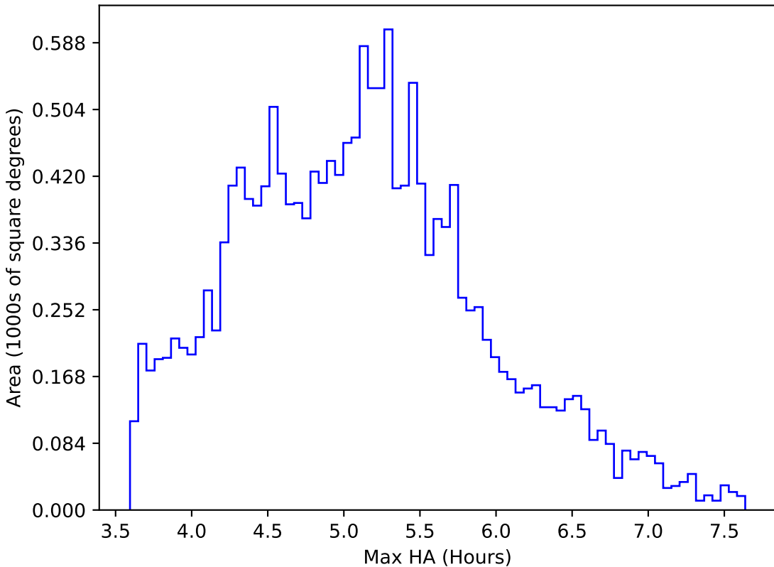
roll_pause_mjdp120_v3.4_10yrs WFD all bands: Max HA
