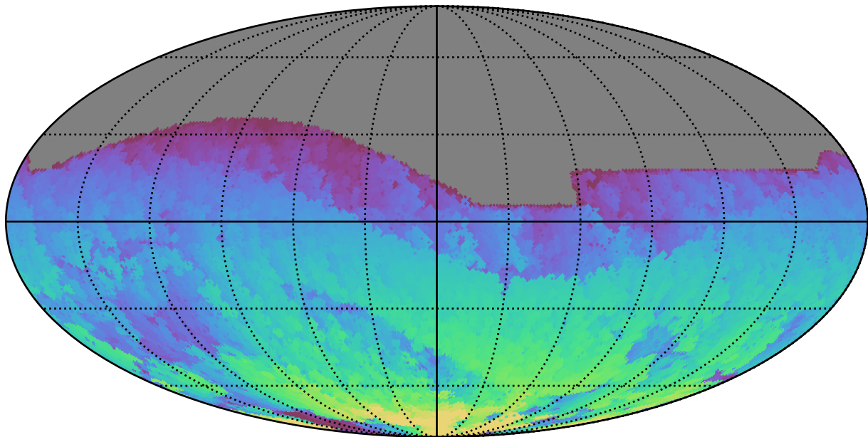
roll_pause_mjdp120_v3.4_10yrs All sky z band: Max HA
