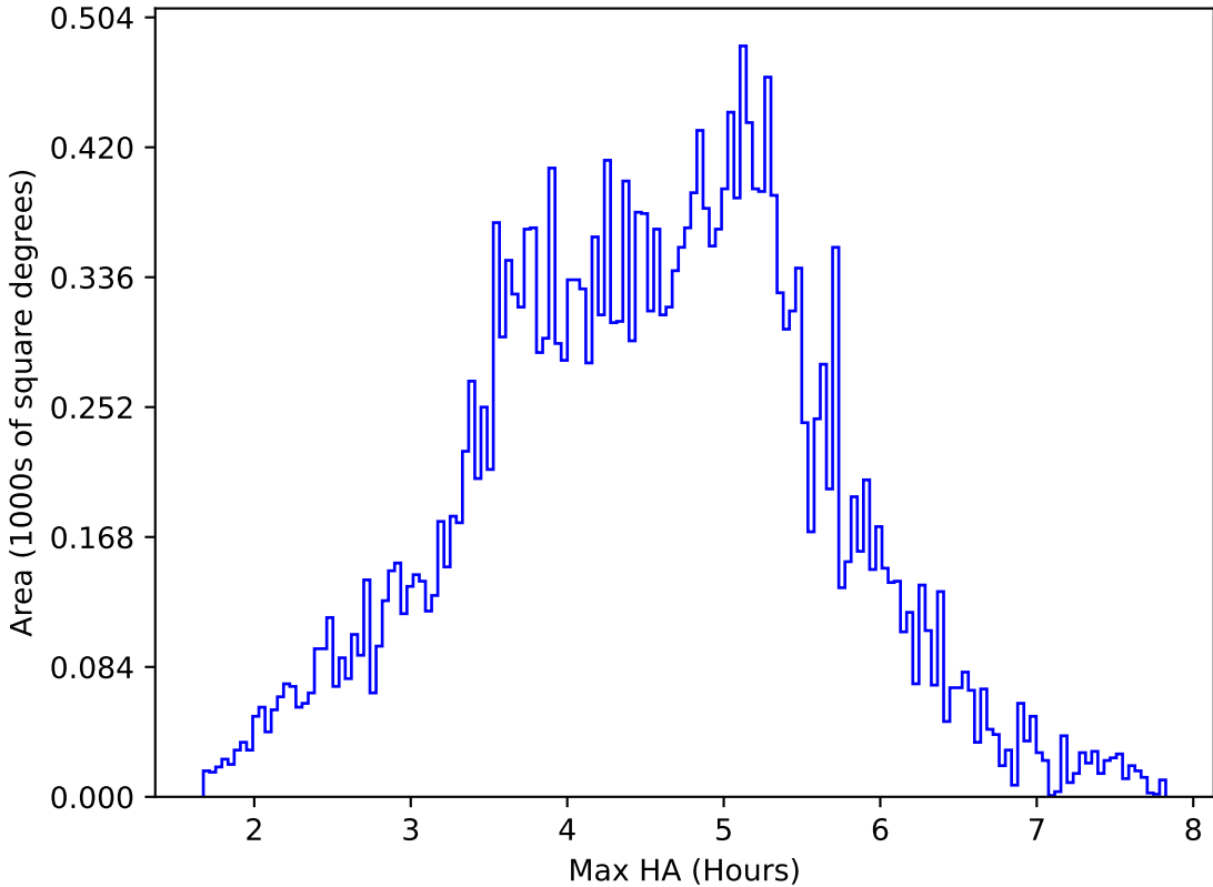
roll_pause_mjdp120_v3.4_10yrs All sky z band: Max HA
