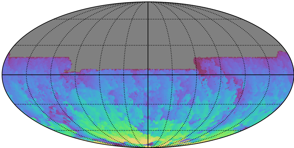
roll_pause_mjdp120_v3.4_10yrs All sky y band: Max HA
