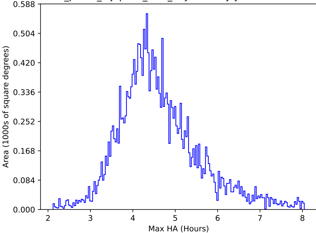
roll_pause_mjdp120_v3.4_10yrs All sky y band: Max HA
