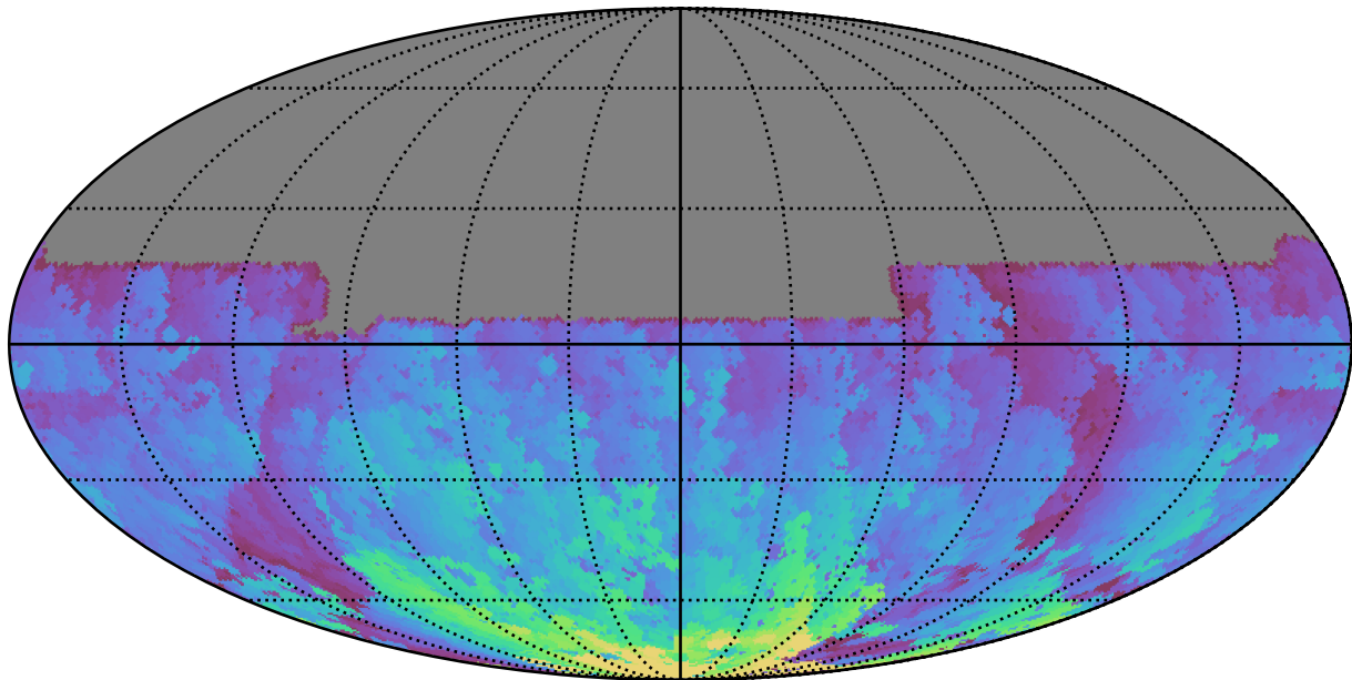
roll_pause_mjdp120_v3.4_10yrs All sky u band: Max HA
