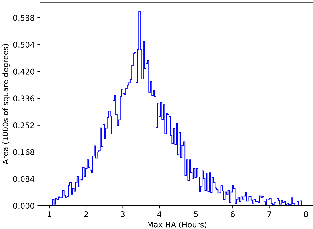
roll_pause_mjdp120_v3.4_10yrs All sky u band: Max HA
