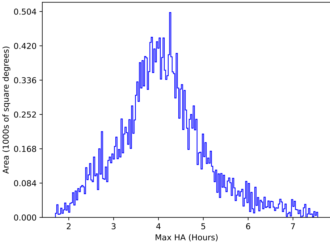
roll_pause_mjdp120_v3.4_10yrs All sky r band: Max HA
