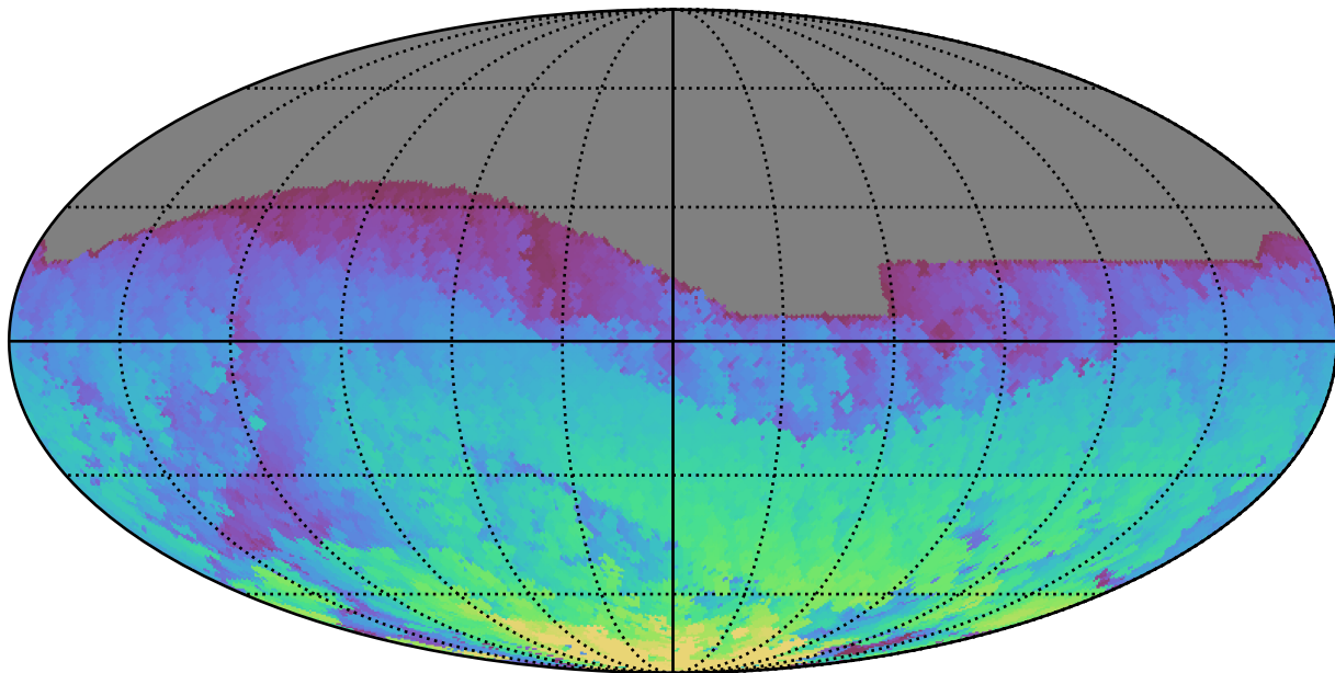
roll_pause_mjdp120_v3.4_10yrs All sky i band: Max HA
