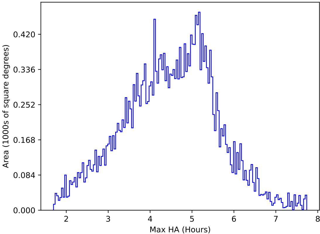
roll_pause_mjdp120_v3.4_10yrs All sky i band: Max HA
