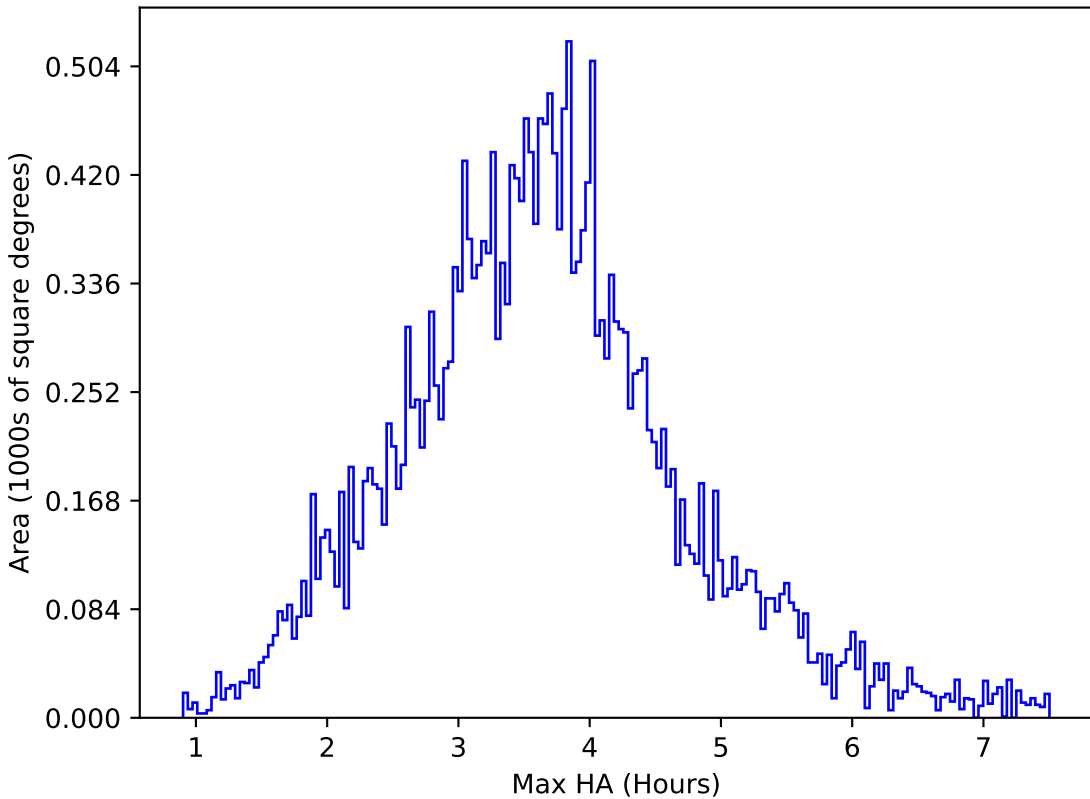
roll_pause_mjdp120_v3.4_10yrs All sky g band: Max HA
