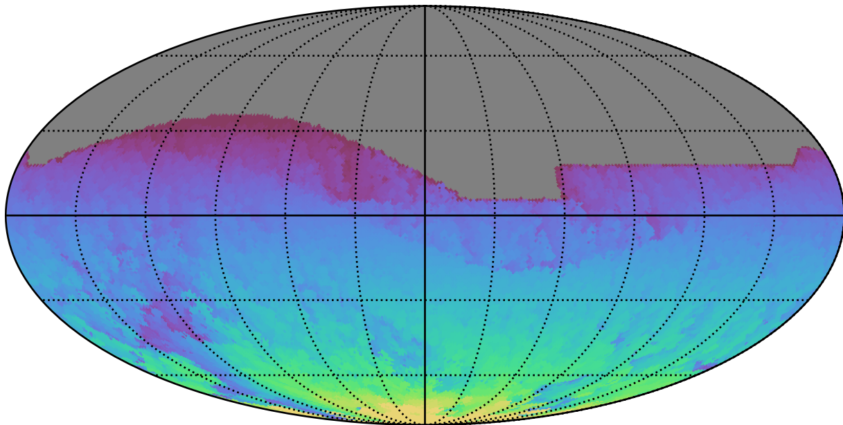
roll_pause_mjdp120_v3.4_10yrs All sky all bands: Max HA
