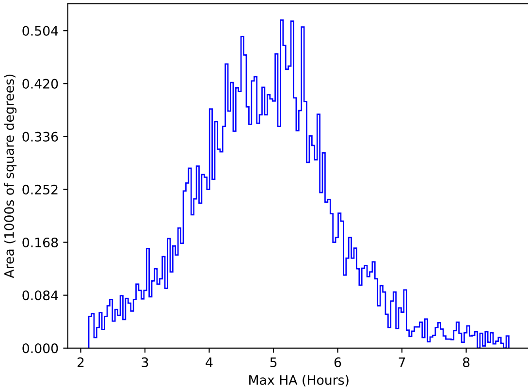
roll_pause_mjdp120_v3.4_10yrs All sky all bands: Max HA
