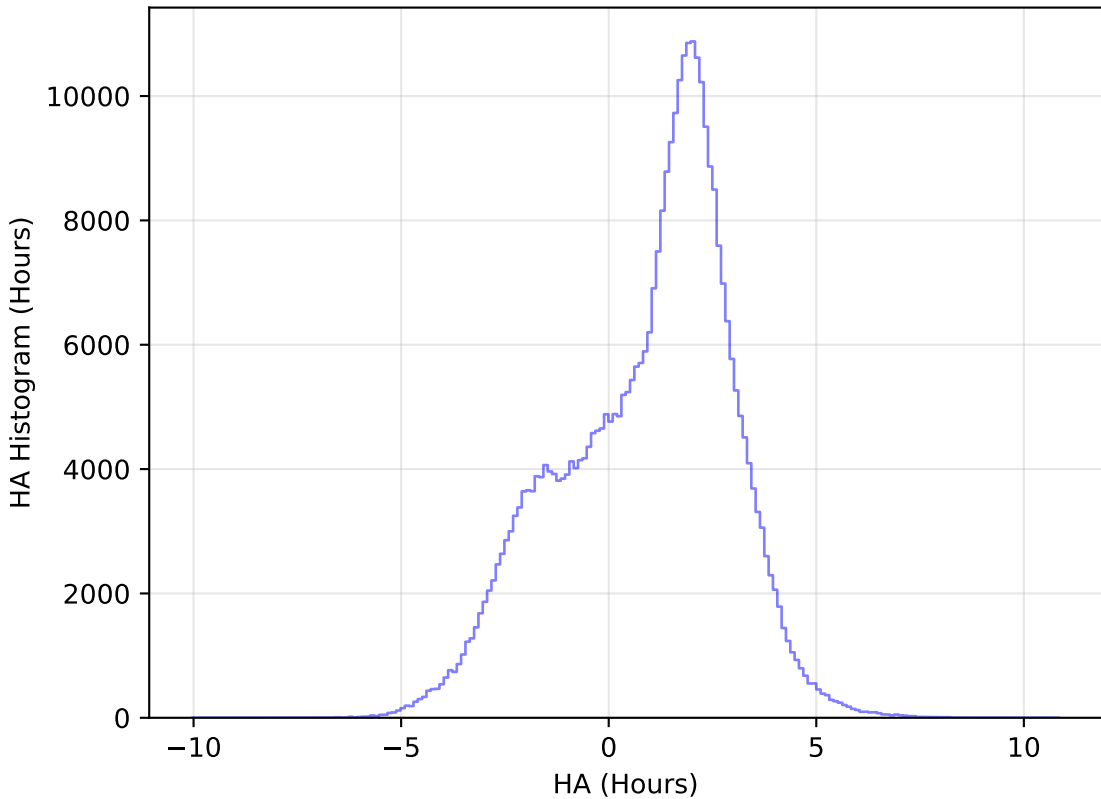
roll_pause_mjdp120_v3.4_10yrs WFD y band: HA Histogram
