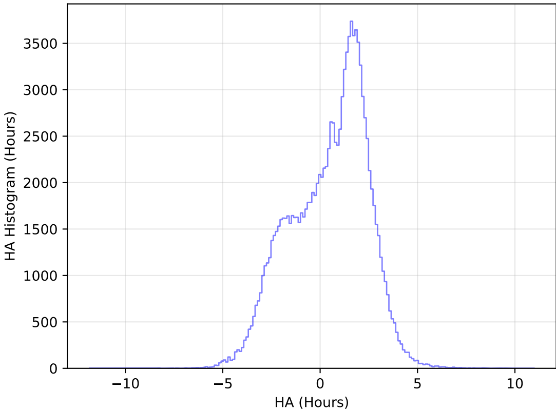
roll_pause_mjdp120_v3.4_10yrs WFD u band: HA Histogram
