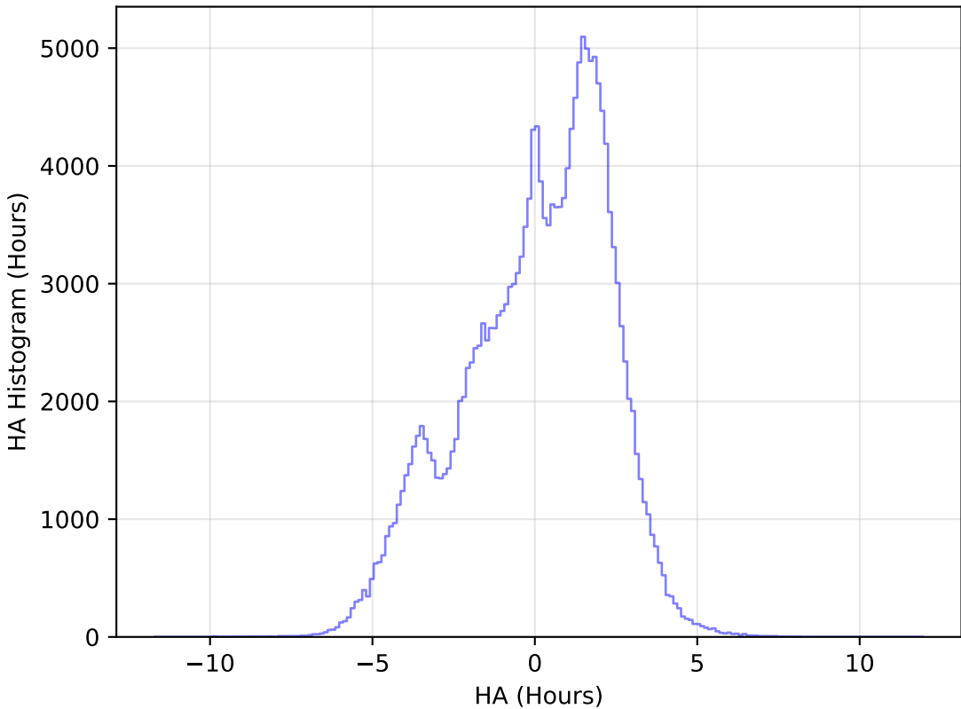
roll_pause_mjdp120_v3.4_10yrs WFD g band: HA Histogram
