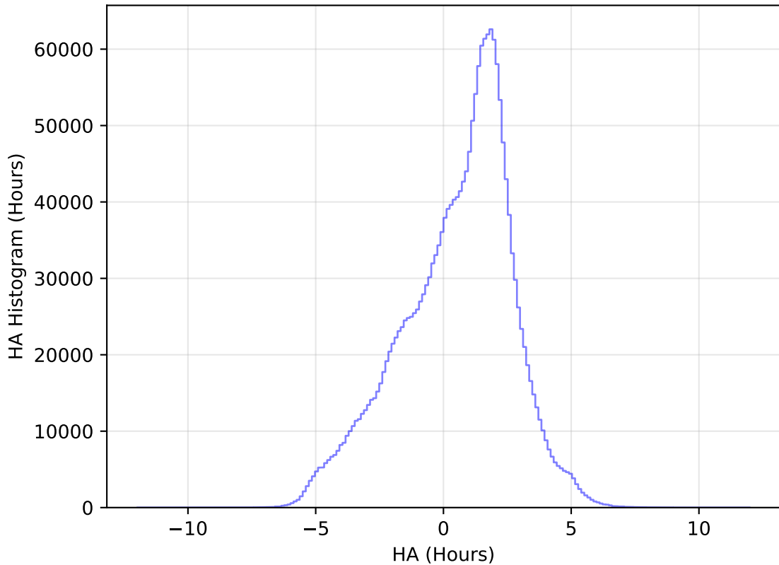
roll_pause_mjdp120_v3.4_10yrs WFD all bands: HA Histogram
